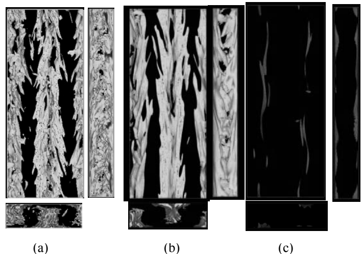
Figure 2 Contour of low-speed streaks; (a) Ha=0 , (b) Ha=8 , (c) Ha=16
