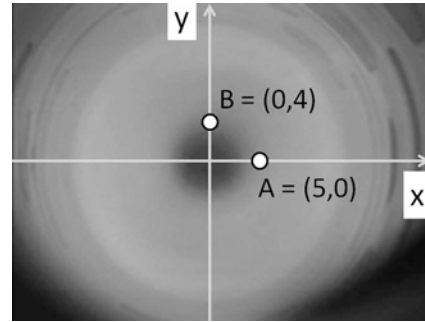
Fig. 1. A CCD image of the plasma hole. Density gradient presents between the dark region in the center and the ambient plasma, i.e. at the position B.
