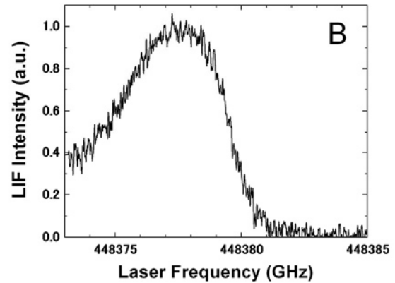
Fig. 3. The LIF spectrum (IVDF) taken at B. Strong asymmetry is evident in the IVDF.
