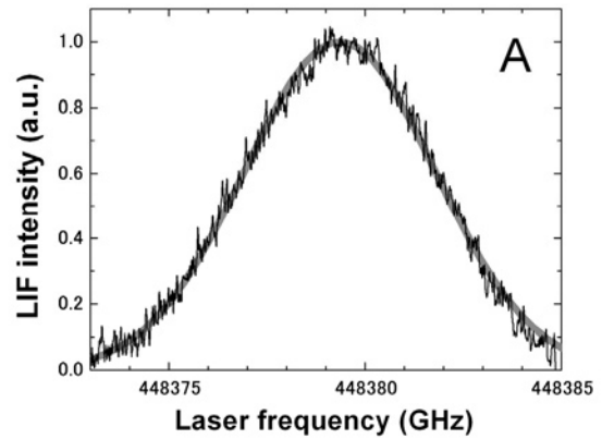
Fig. 2. The LIF spectrum (IVDF) taken at A.
