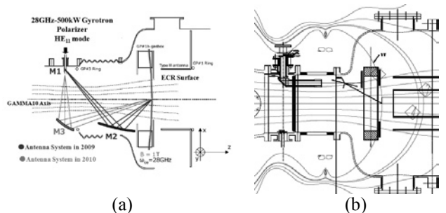
Fig.3 Scheme of the central ECH antenna system (a) in 2009 and 2010, (b) new design.
