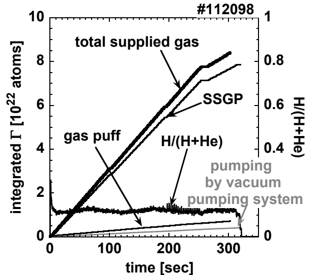
Fig. 2. Estimated amount of flow during the five-minutes operation. Supplied amount of gas puff and SSGP, total supplied amount, and evacuated amount by the vacuum pumping system are plotted. hydrogen ion ratio is also plotted.
