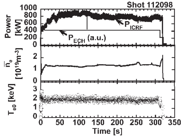
Fig. 1. Time evolution of the plasma parameters for the analyzed five-minutes operation. Injected power, line-averaged electron density, and central electron temperature are plotted from top column.
