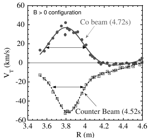
Fig. 1: Profiles of V_T in the case of B > 0 configuration with co-beam injection (circle) and counter-beam injection (square).
