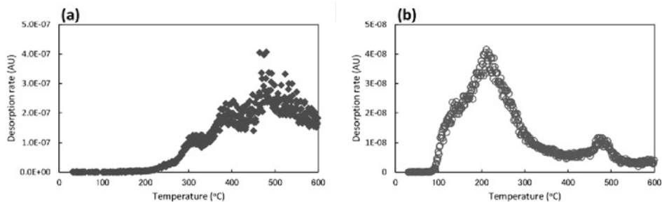
Fig. 2. Thermal desorption spectra of H 2 , (a), and He, (b) for F82H irradiated with hydrogen/helium mixed plasma.
