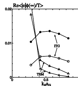
Figure 2: Residual zonal flow as a function of k_0 \rho_i , which are generated by ITG modes and TEMs.
