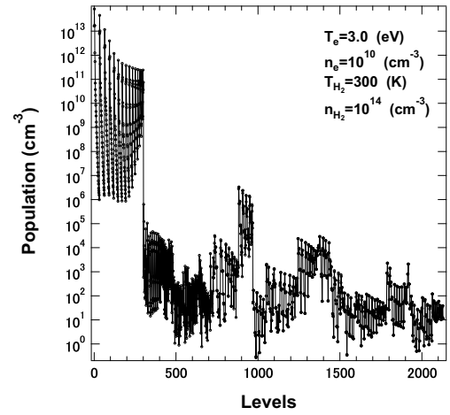
Fig. 1: Calculated population (see Table I).
