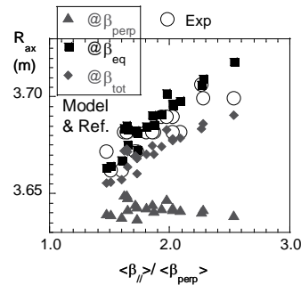
Fig. 1 The measured Shafranov shift as the function of the anisotropy of the pressure.
