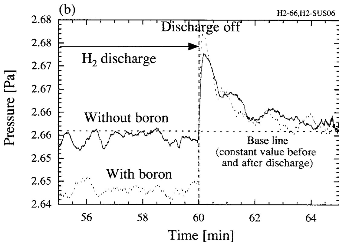
Fig.2. Time evolution of hydrogen pressure during H 2 discharge after H evacuation (stage (I)), with a SS liner with and without B-coating. (a) total discharge time and (b) around the end of discharge are indicated.
