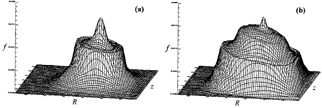
FIG. 2. Fast ion distribution as a function of R and z averaged in the toroidal angle with v = v_A for (a) P_o=2\% , \tau_s = 100\tau_A , t=900\tau_A , and (b) P_o=4\% , \tau_s = 1000\tau_A , t=2800\tau_A .
