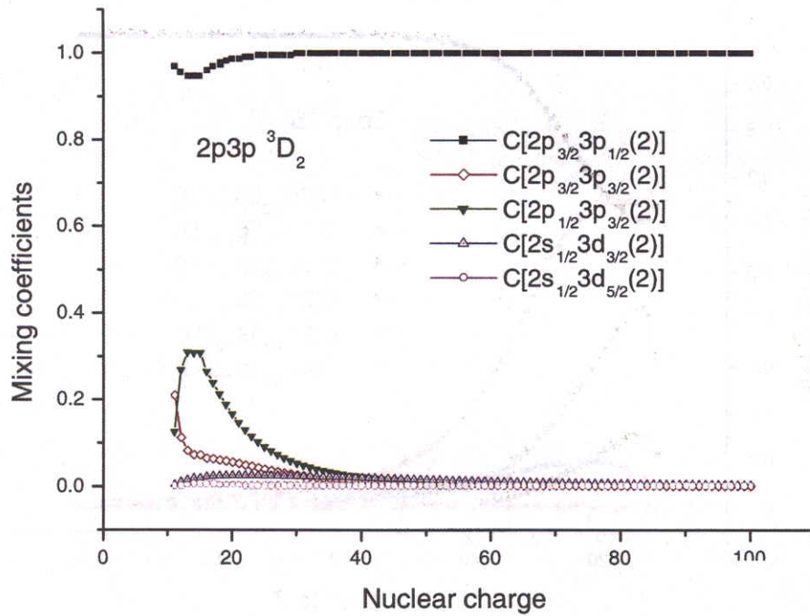
FIG. 8. Mixing coefficients for the 2p3p\ ^3D_2 level as functions of Z
