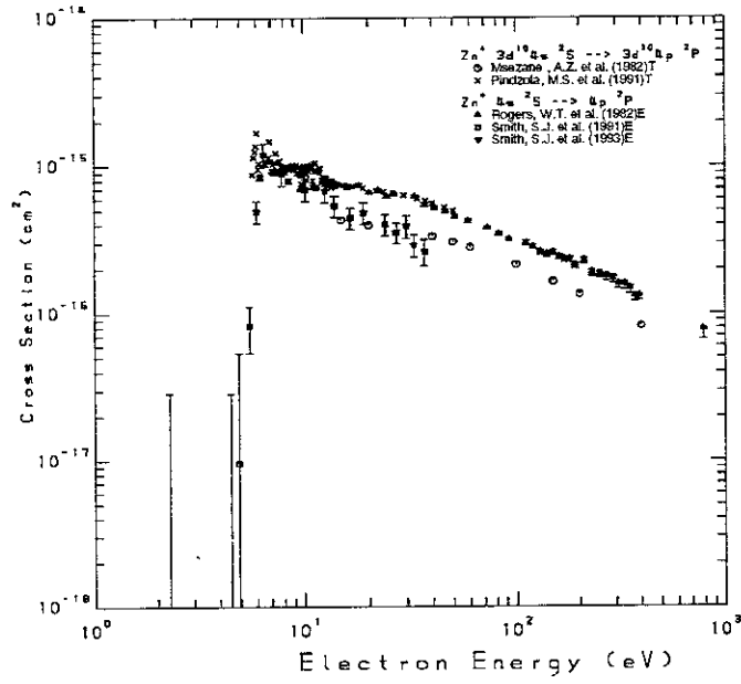
Figure 12: Excitation cross section of \text{Zn}^+ by electron impact.
