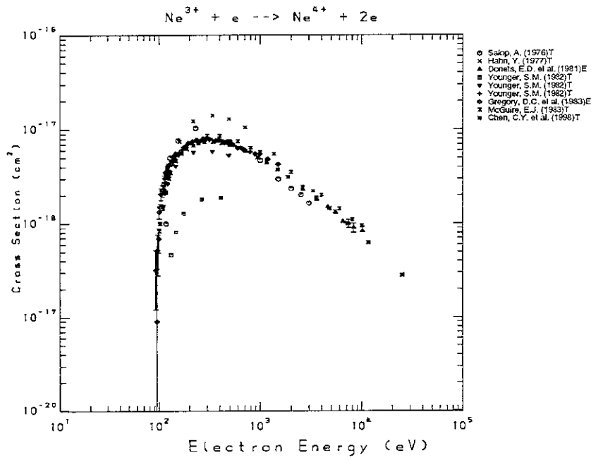
Figure 7: Ionization cross section of \text{Ne}^{3+} by electron impact.
