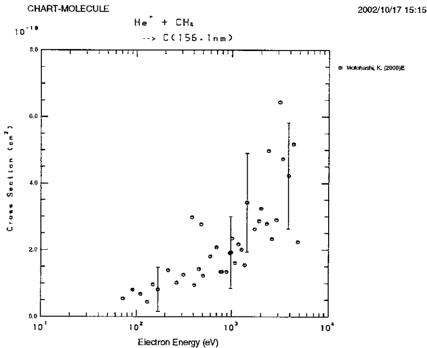
Figure 26: Emission cross section of carbon λ 156.1nm spectral line produced in He + + CH 4 collision. This graph is from new database for molecules (CMOL, i.e. Chart-MOLecule) which is now in preparation.
