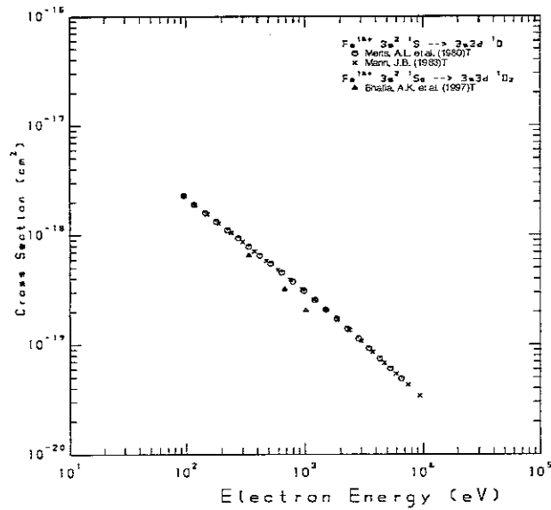
Figure 4: Excitation cross section of \text{Fe}^{22+} by electron impact.
