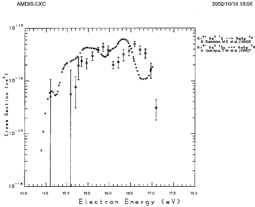
Figure 11: Excitation cross section of \text{Kr}^{6+} by electron impact.
