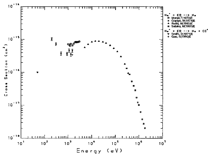
Figure 20: Charge transfer cross section of \text{He}^+ + \text{CO} collision.
