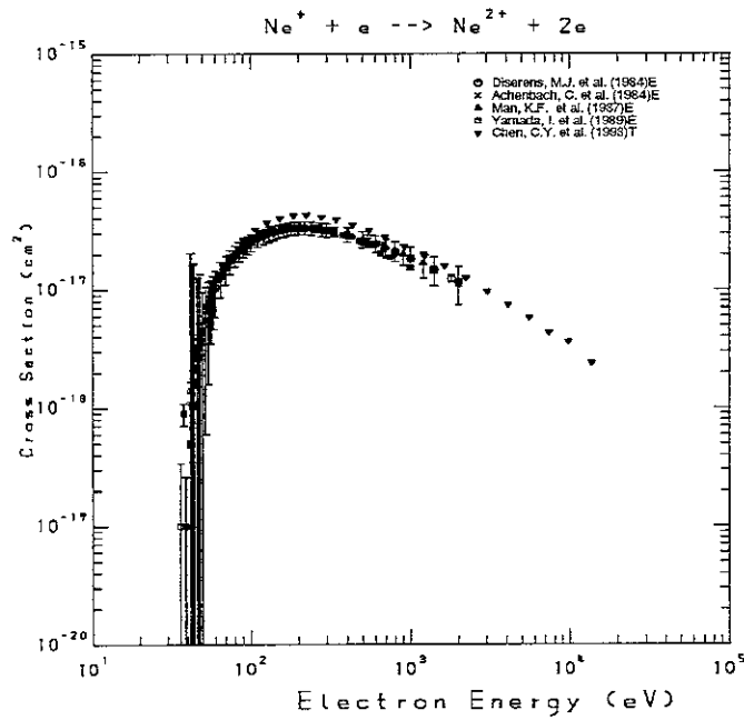
Figure 8: Ionization cross section of \text{Ne}^{+} by electron impact.
