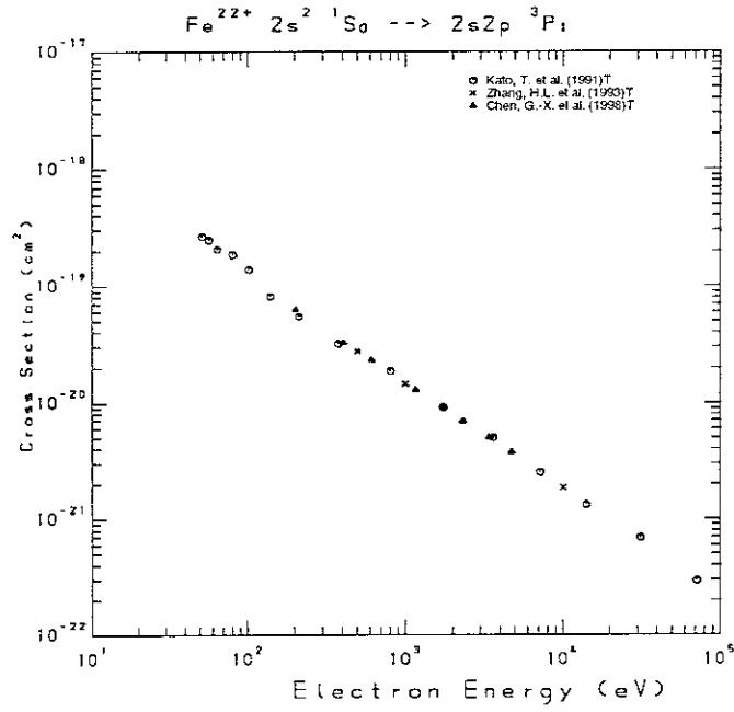
Figure 3: Excitation cross section of \text{Fe}^{22+} by electron impact.
