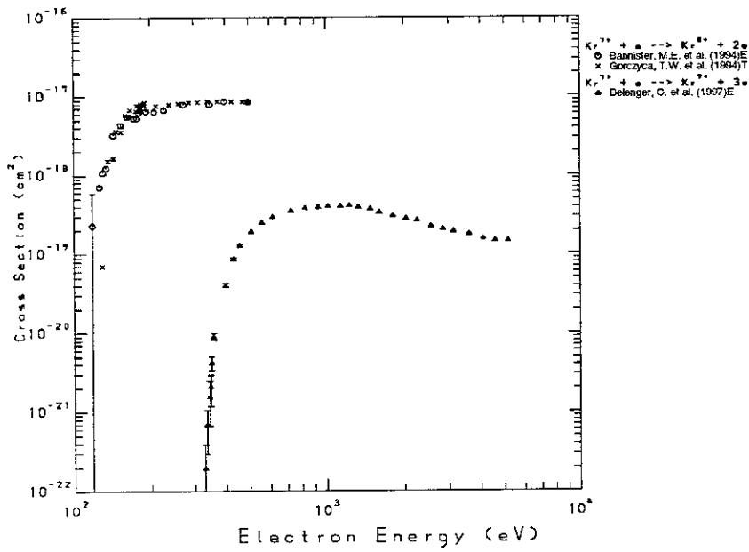
Figure 13: Ionization cross section of \text{Kr}^{7+} by electron impact.
