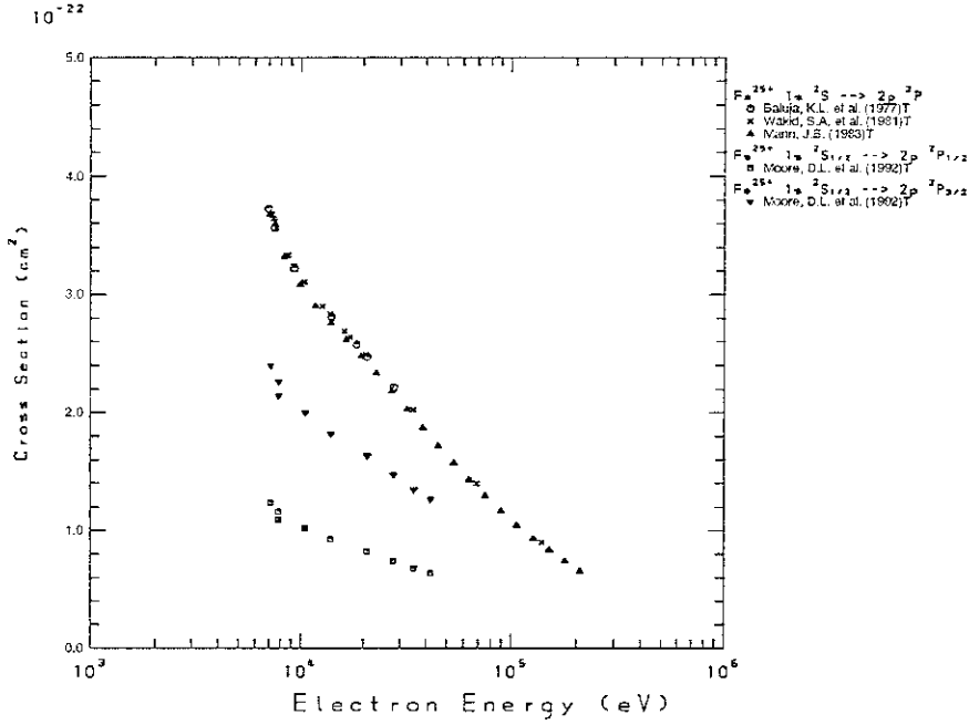
Figure 2: Excitation cross section of \text{Fe}^{25+} by electron impact.
