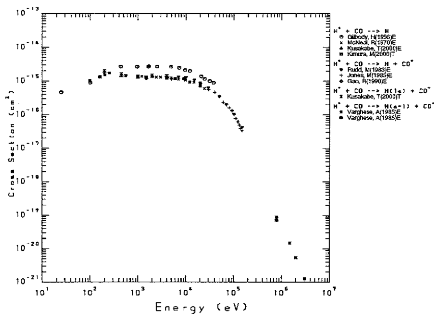
Figure 19: Charge transfer cross section of \text{H}^+ + \text{CO} collision.
