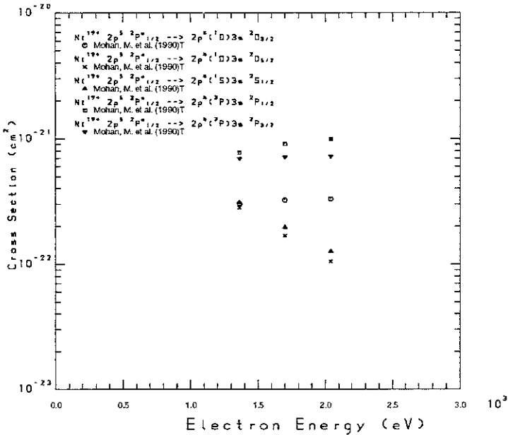
Figure 9: Excitation cross section of \text{Ni}^{17+} by electron impact.
