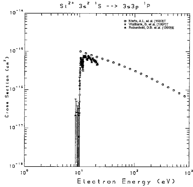
Figure 10: Excitation cross section of Si 2+ by electron impact.
