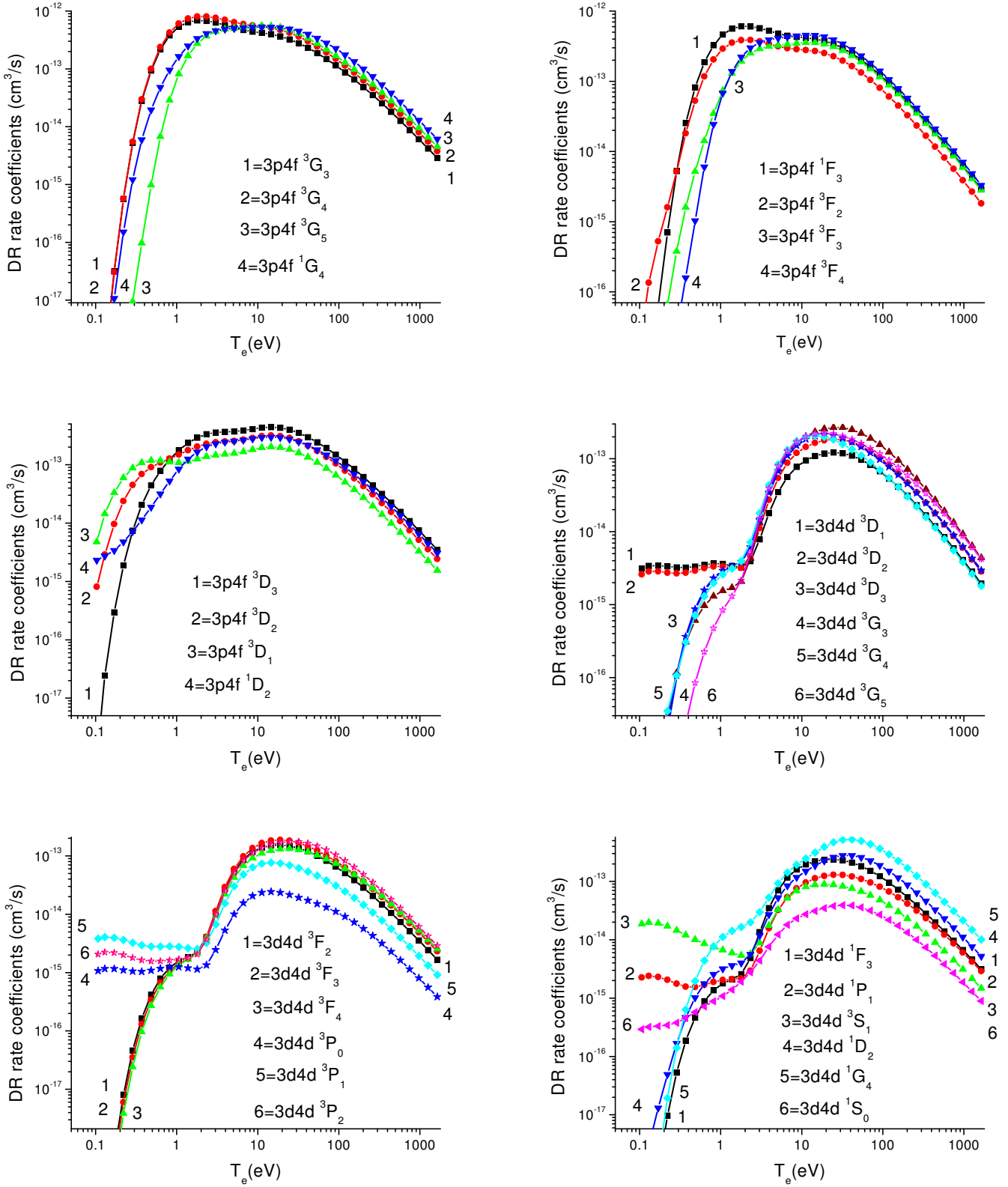
FIG. 8: Dielectronic Recombination rate coefficient \alpha_d(\gamma|3s) for the 3l4l' even-parity states as a function of T_e in Mg-like Fe.
