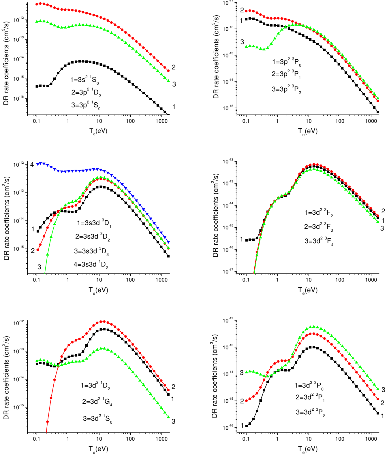
FIG. 6: Dielectronic Recombination rate coefficient \alpha_d(\gamma|3s) for the 3l3l' even-parity states as a function of T_e in Mg-like Fe.
