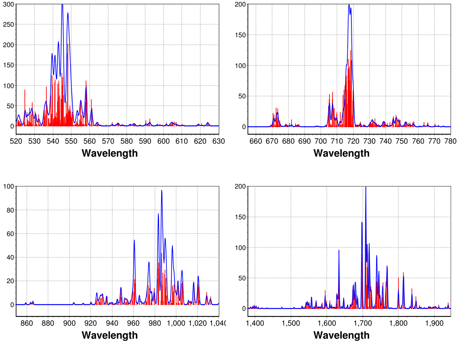
FIG. 2: Synthetic spectra of dielectronic satellite lines from \text{Fe}^{14+} ion at T_e = 10 eV for \lambda = 520 - 2000 Å. Resolution power, R = \lambda/\Delta\lambda = 700 is assumed to produce a Gaussian profile. The scale in the ordinate is in units of 10^{-15} \text{ cm}^3/\text{s} .
