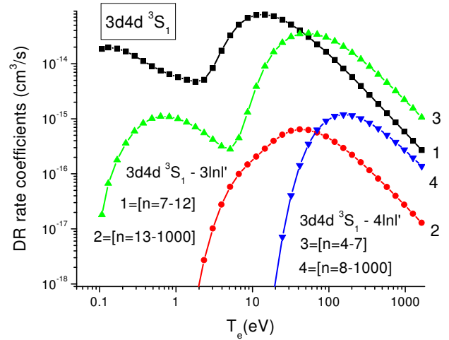
FIG. 5: Contribution of the 3lnl' and 4lnl' states to the Dielectronic Recombination rate coefficient \alpha_d(\gamma|3s) for even-parity states as function of T_e in Mg-like Fe.
