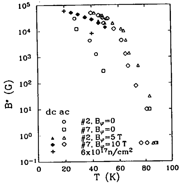
Fig.7.2-6 The irreversibility field B^* vs. T for the \text{Bi}_2\text{Sr}_2\text{CaCu}_2\text{O}_8 single crystals before and after irradiation with heavy ions to the fluences shown. Results from ac studies (open symbols) and dc magnetization measurements (filled symbols) are shown; data from neutron damage investigation are included for comparison (crosses). (from Ref.13 fig.2)
