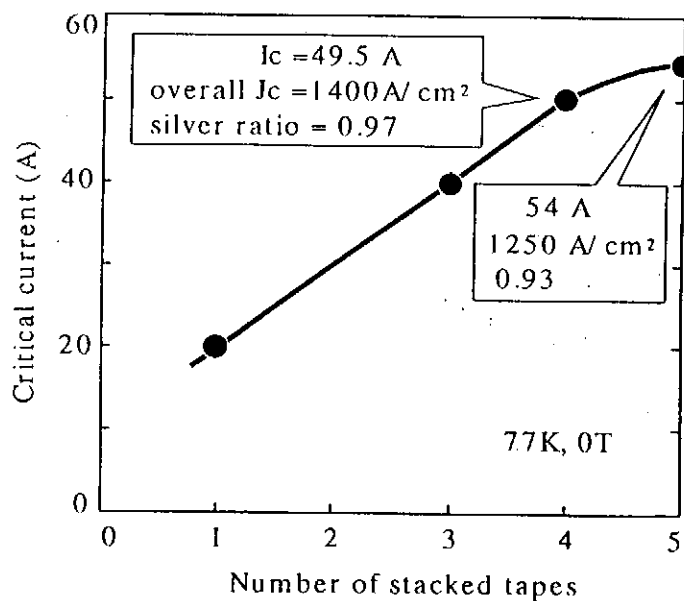
Fig.5.1-16 Critical current vs. number of stacked Tl-1223 tapes.
