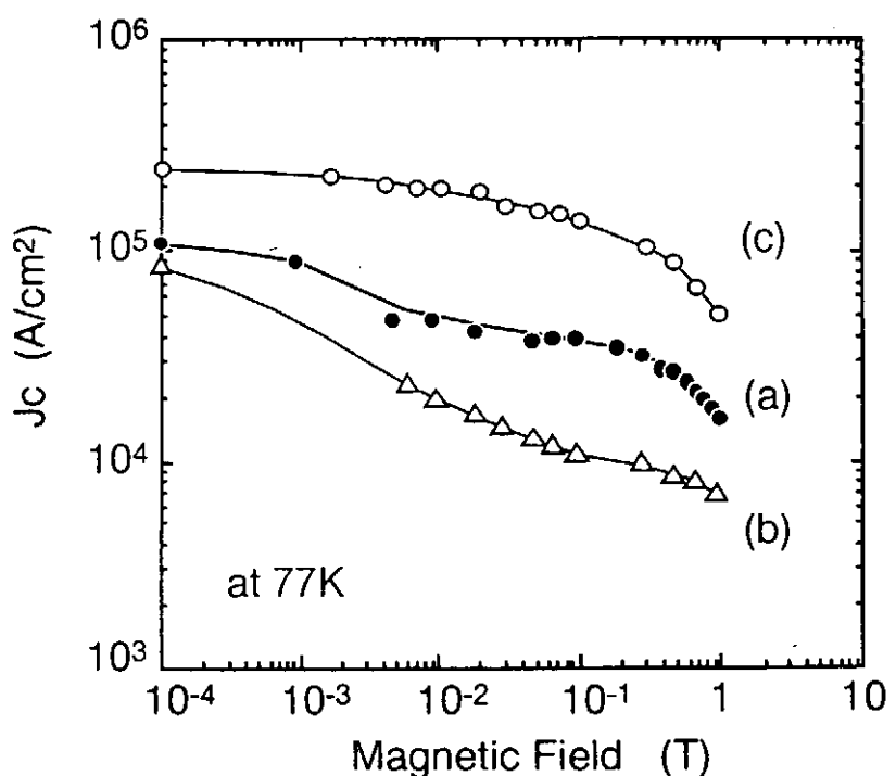
Fig.5.1-12 Magnetic field dependences of J_c for TlBa 2 Ca 2 Cu 3 O x films deposited (a) on the cube-textured silver tape and (b) on commercial silver tape, and (c) TlBa 1.6 Ca 0.4 Cu 3 O x film deposited on SrTiO 3 (100) substrate with the field applied parallel to the c-axis.
