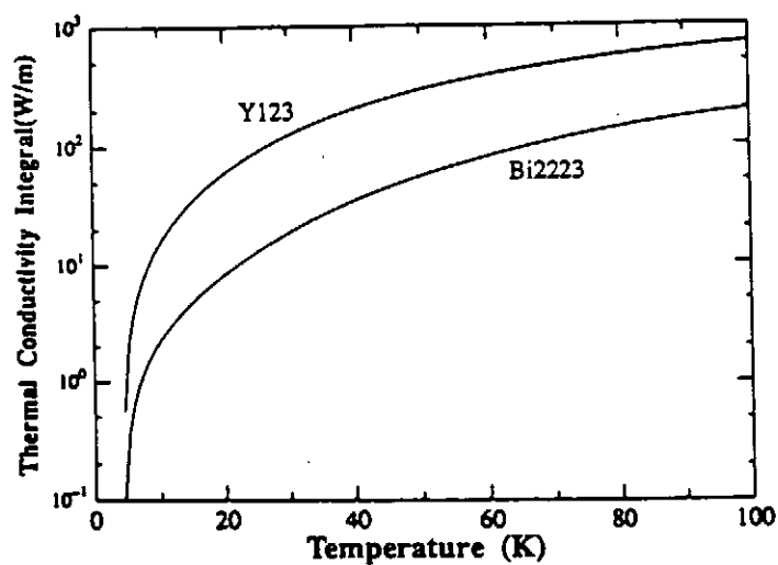
Fig.9.1-2 Comparison of thermal conductivity integral for a melt processed Y-123 rod and a powder sintering Bi-2223 tube.
