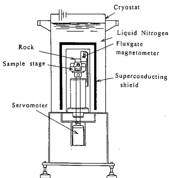
Fig.11.6-4 Superconducting magnetic shielded rock magnetometer.
