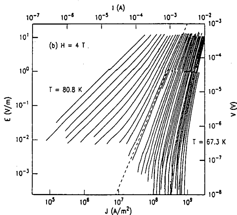
Fig. 2.3.3-1 Current-voltage (I-V) curves at constant temperatures for H = 4T .
