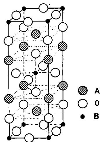
Fig.2.2-2 K 2 NiF 4 structure of (La,Ba) 2 CuO 4 Superconductor
