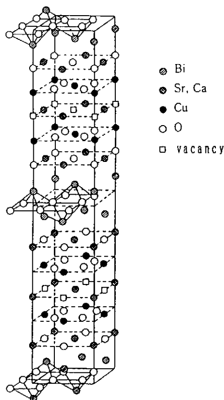
Fig.2.2-4 Pseudo tetragonal structure of low T_c phase( \text{Bi}_2\text{Sr}_2\text{CaCu}_2\text{O}_{8+x} ) of Bi-based oxide superconductors
