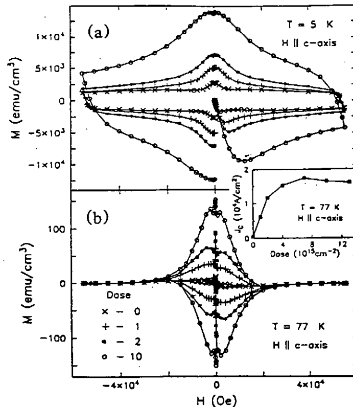
Fig.7.2-12 Magnetization M(H) vs. magnetic field of Y-Ba-Cu-O crystal No.3 for different doses of 3-MeV proton irradiation, at (a) T=5\text{ K} and (b) T=77\text{ K} . Inset: Dose dependence of the critical current at 77 K and 1 T. The doses are given in unit of 10^{15}\text{ protons/cm}^2 .(from Ref.12 fig.1)
