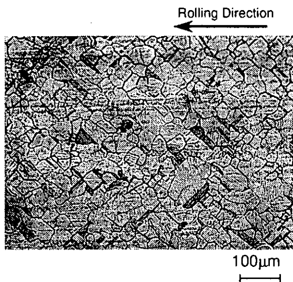
Fig.5.1-8 Surface of cube-textured silver tape.
