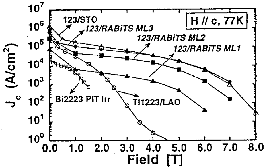
Fig.4.3-3 Magnetic field dependese of J_c of in-plane aligned YBCO tape by Rolling Assisted Bi-axially Aligned Ni tape (25).
