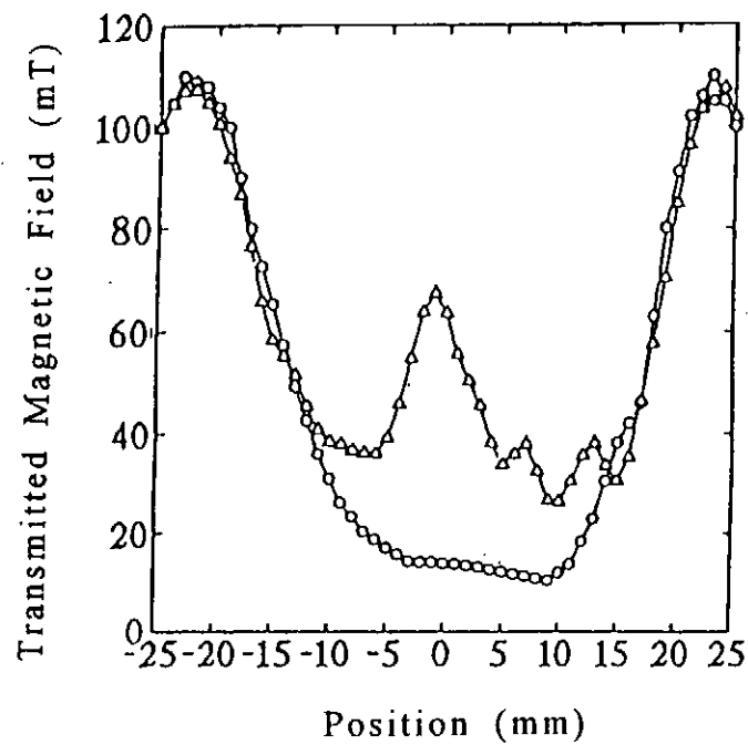
Fig.11.8-3 Magnetic flux density distribution.
