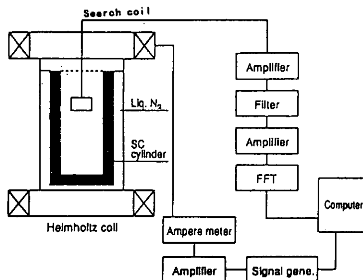
Fig.11.3-1 Measurement of magnetic shielding.
