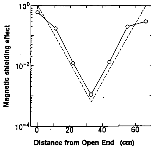
Fig.11.5-3 Magnetic shielding effect vs. distance from the open end of the shielding vessel. ○:experimental,-----:theoretical. External magnetic field : 0.01 mT, 13.5 Hz.
