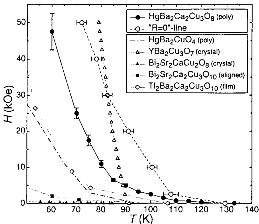
Fig. 2.3.2-2 Irreversibility boundaries for various copper-containing superconductors. The temperatures where R(H, T) is zero within the accuracy of the measurement for a \text{HgBa}_2\text{Ca}_2\text{Cu}_3\text{O}_8 polycrystalline sample are drawn for comparison.
