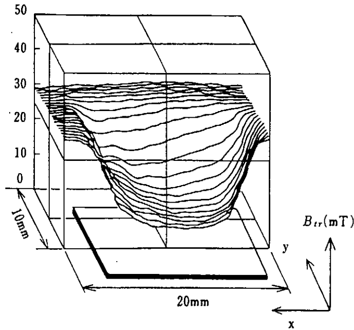
Fig.11.8-4 Three-dimensional distribution of flux density over the half sample surface.
