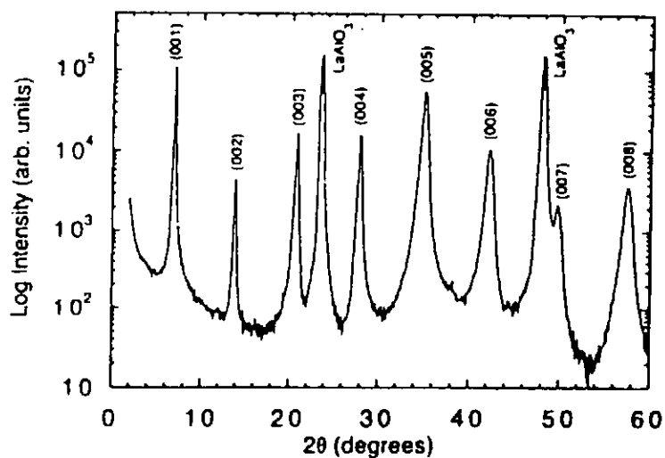
Fig.5.1-24 \theta-2\theta X-ray diffraction scan (using \text{CuK}\alpha radiation) of a "phase pure" in situ \text{TlBa}_2\text{CaCu}_2\text{O}_7 film deposited on \text{LaAlO}_3 .
