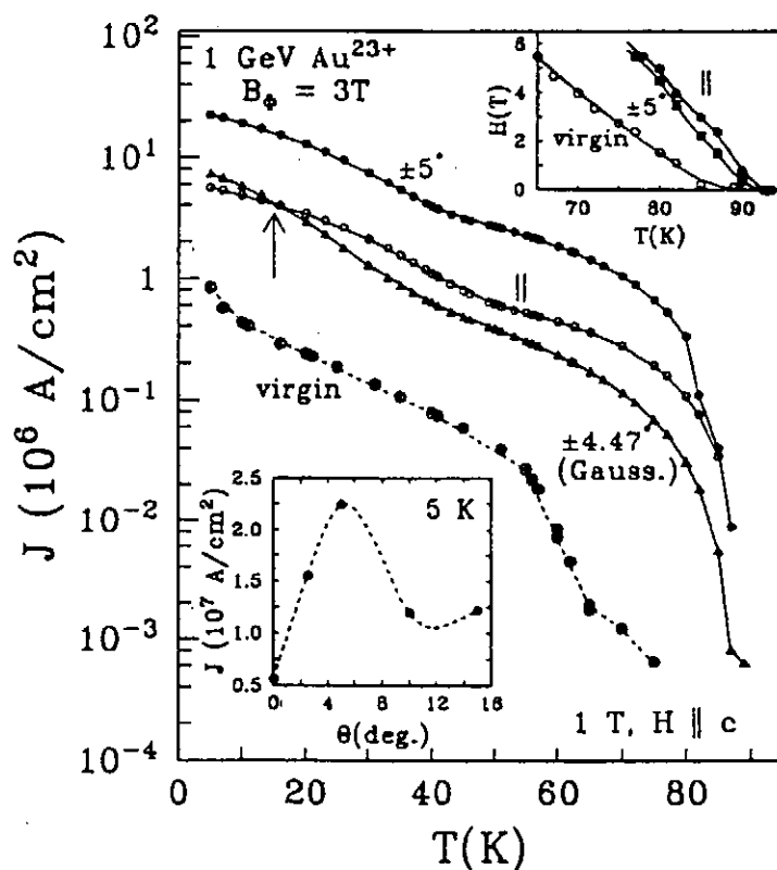
Fig.7.2-11 Persistent current density J(T) for YBCO crystals with three splay configurations of columnar pins, each with B_\phi = 3\text{ T} : planar splay (solid dots) with \Theta=\pm 5^\circ , parallel tracks (open circles), and a Gaussian distribution (solid triangles) with the full width at half maximum of \pm 4.47^\circ . The best result is for the \pm 5^\circ planar splay (also lower inset).
