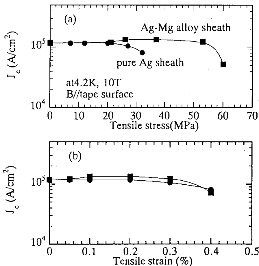
Fig.7.1-3 (a) critical current density vs. tensile stress and (b) critical current density vs. tensile strain curves at 4.2K and 10T for Bi-2212 multilayer tapes.
