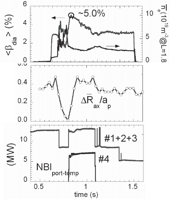
Fig.1 The waveform of the \langle\beta_{dia}\rangle=5.0\% plasma. (a) the averaged beta value and the line averaged electron density. (b) the normalized magnetic axis shift. (c) the port-through NBI power.
