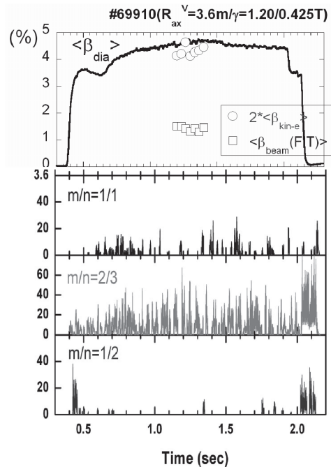
Fig.2 The waveform of the \langle\beta_{dia}\rangle=4.8\% plasma. (a) the averaged beta value and the beam component. (b)-(d) the mode amplitude of the magnetic fluctuations.
