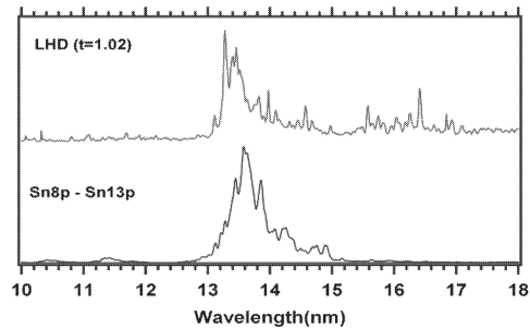
Fig. 2 Emission of \text{Sn}^{10+} from CXs and FAC
