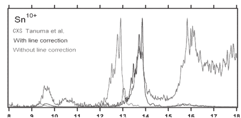
Fig. 2 Emission of \text{Sn}^{10+} from CXs and FAC
