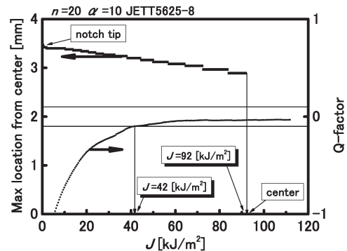
Fig.1 Q-factor and MAX location VS. J
