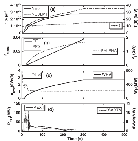
Fig. 2 Temporal evolution of plasma parameters with the pre-programming power of P_{\text{EXT-pre}}=25 MW and \tau_{\text{rise}}=300 sec.
