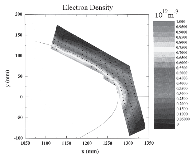
Fig. 2. Two-dimensional electron density profile reconstructed from the emission profile.
