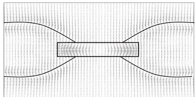
Fig. 2. Vector plots of electron flow velocity in (x,y) plane at \omega_{ce}t=355 .
