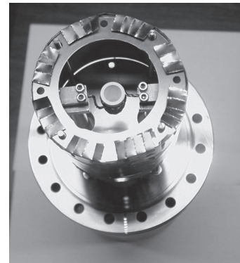
Fig. 1 Test bench of lithium oven
