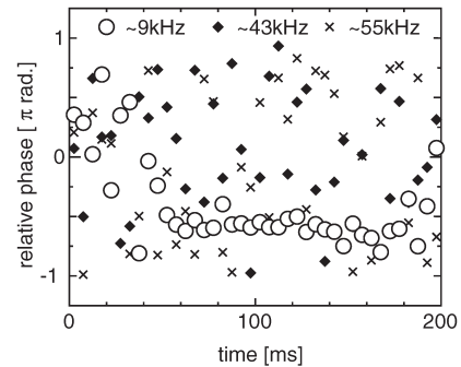
Fig. 2. Time evolution of relative phase between density fluctuations in the azimuthal direction.
