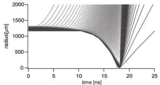
Fig. 1 Radius vs. time diagram of implosion simulation with pellet gain G=100 .
