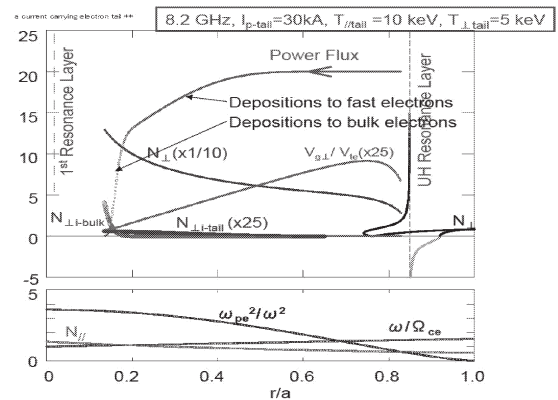
Fig.2 Propagation and absorption of EBW in a QUEST plasma
