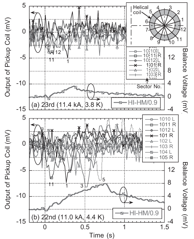
Fig. 2. Output of pickup coils and balance voltage of the helical coils during the (a) 23rd and (b) 22nd propagation of a normal zone.
