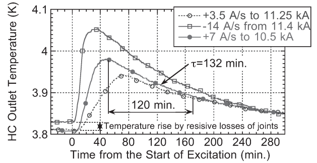
Fig. 1. Temperature rises at the helical coil outlet.
