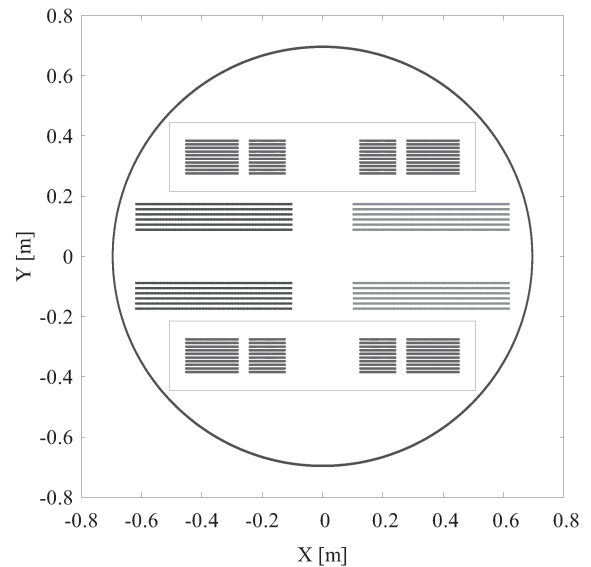
Fig. 2. Layout of the enhancement superconducting and split superconducting coil which can generate 4 T on the mid-plane.
