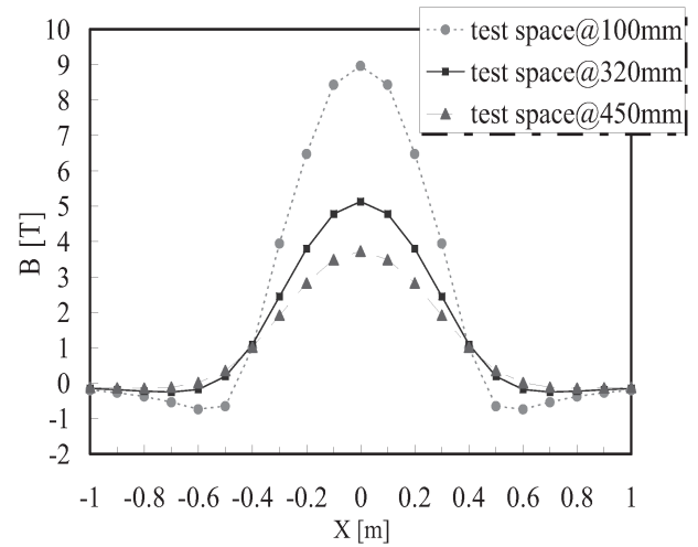
Fig. 1. Magnetic field distributions, which are generated by the split coil with each test space, on the mid-plane.
