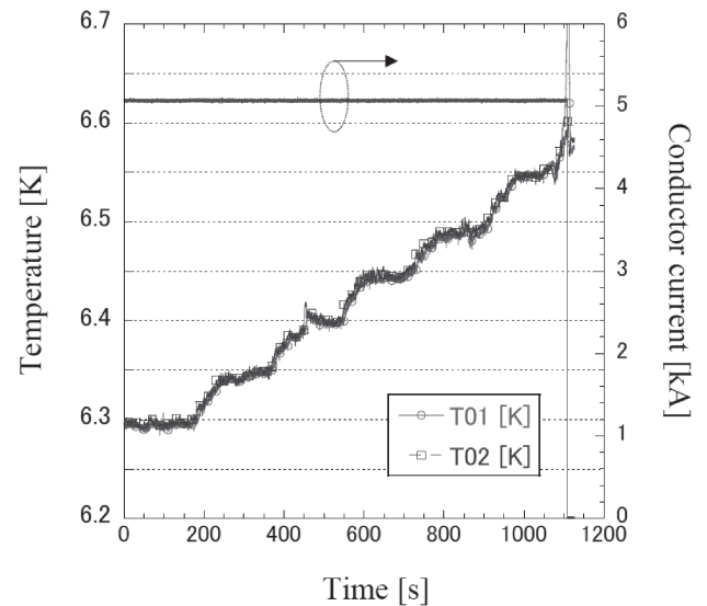
Fig. 2. Current value and temperature profiles of the conductor in the test to measure current sharing temperature (Tcs). T01 and T02 show the temperature measured by CERNOX thermometer, which is attached on a conduit on the test conductor.
