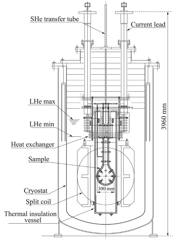
Fig. 1. Schematic view of the upgraded NIFS superconductor test facility
