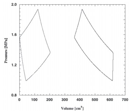
Fig. 2 P-V diagram of the pulse-tube
