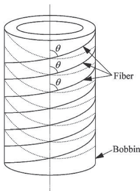
Fig 1. Fiber winding angle in bobbin.
