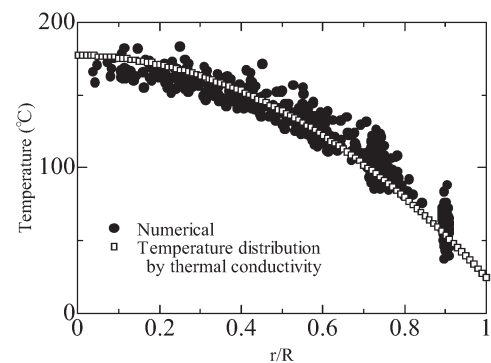
Fig. 3 Temperature distribution in the case with volumetric heating
