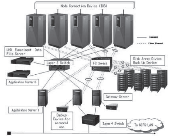
Fig. 1: Schematic View of LHD Numerical Analysis System
