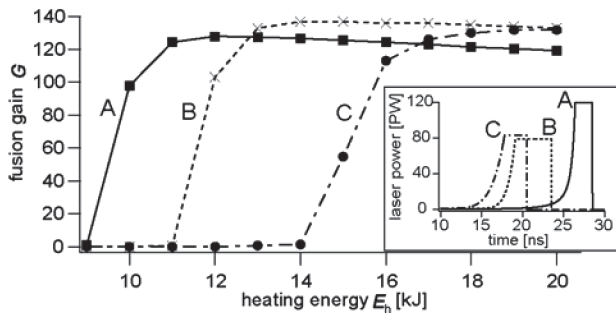
Fig. 2 Fusion gain G versus heating laser energy for various waveform of the implosion laser.
