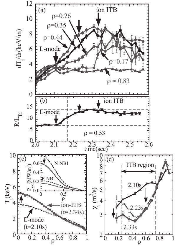
Fig. 1: Time evolution of (a) ion temperature gradients at various normalized radii and (b) R/L_{Ti} during the formation of an ITB and (c) radial profiles of ion temperature and deposition power to ions by P-NBI and N-NBI at t = 2.1 s (L-mode : dashed lines) and t = 2.34 s (ion-ITB : solid lines) and (d) radial profiles of ion thermal diffusivity at t = 2.10 s (L-mode), t = 2.23 s (early phase of ion-ITB) and t = 2.33 s (later phase of ion-ITB) in the discharge with carbon pellet injection (#90982)
