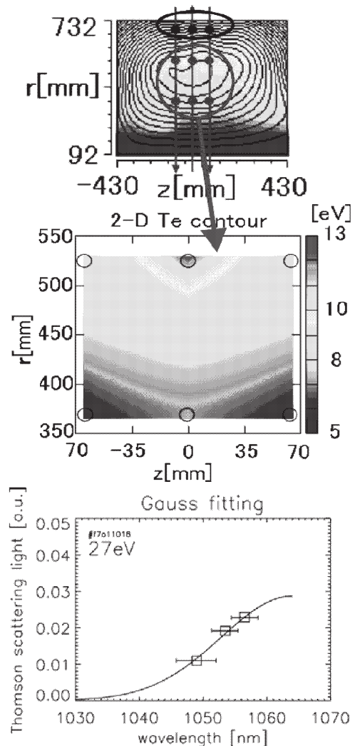
Fig. 1 The laser beam path and measurement points for the present 3x3 2-D Thomson scattering measurement in the poloidal flux contour of ST plasma (top), the measured 2-D contour of electron temperature (middle) and the Thomson scattered lights as a function of wavelength for Gaussina fitting (bottom).
