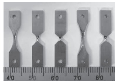
Fig. 1 Photos of the miniature size hourglass specimen (( \phi , \phi/\rho ) = (1.25, 0.125), (1.25, 0.500), (1.25, 1.000) (1.85, 0.125), (1.85, 1.000) from left side)
