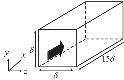
Figure 1 Computational domain.
