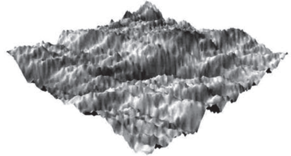
Fig. 2 Fractal surface with fractal dimension 2.3
