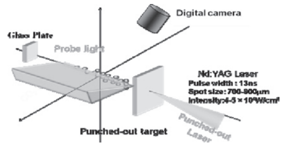
Fig.1 Experimental setup
