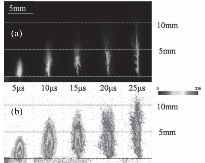
Fig.2 (a) Time-elapsd images of light scattering by lead particles. (b) Intensity distribution of each scattering image.
