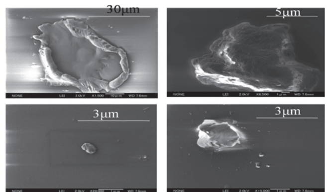
Fig.3 Scanning electron microscope (SEM) images of ablated particles captured on a glass plate placed 25 mm from the target.
