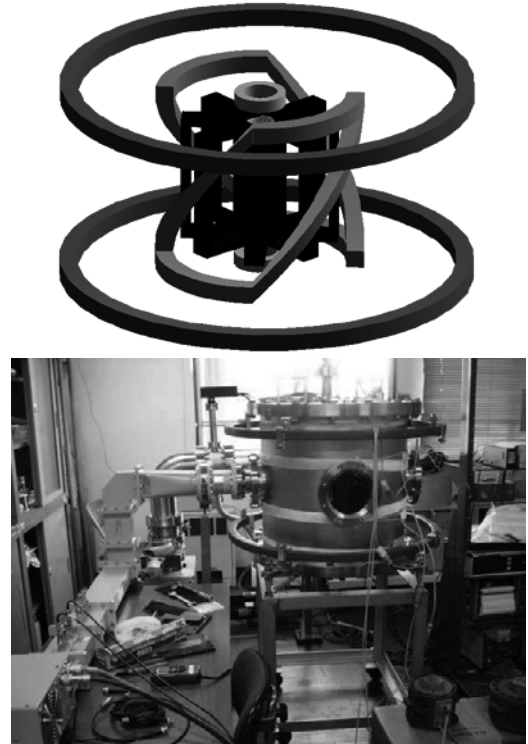
Fig.1 TOKASTAR -2 machine (Upper) Coil configuration concept inside vacuum chamber, (Lower) Experimental setup photo.
