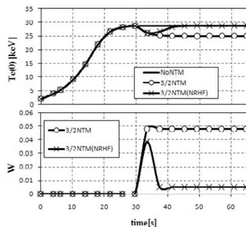
Fig. 2 Time evolution of central temperature T_e(0) and the 3/2 NTM normalized island width W . The case of non-resonant external helical field application is also shown as 3/2NTM(NRHF).
