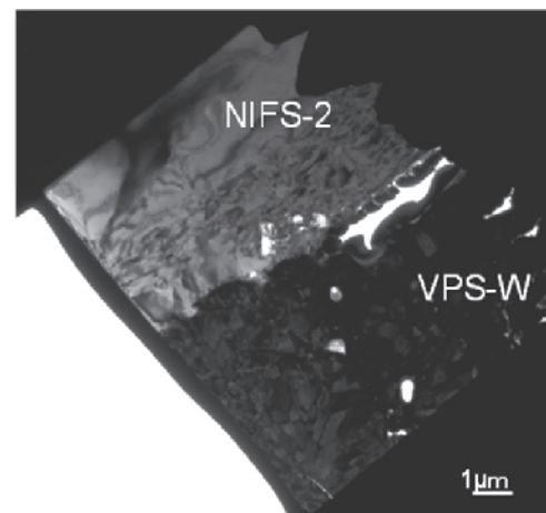
Fig. 1. Microstructure of interface between NIFS-HEAT-2 and VPS-W.
