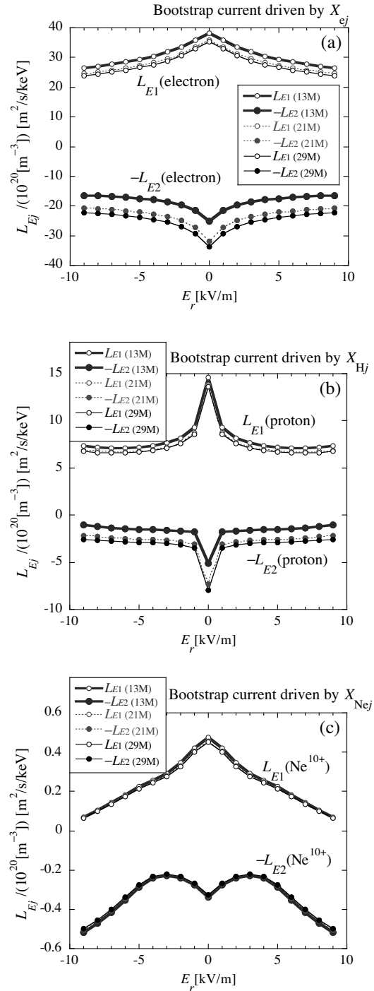
Fig.1 The bootstrap current and Ware pinch coefficients obtained by the 13M, 21M, and 29M approximations for a e^-+H^++Ne^{10+} plasma in a LHD configuration with R_{\text{ax}}=3.6\text{m} , B=2.45\text{T} (at r/a=0.5 ).
