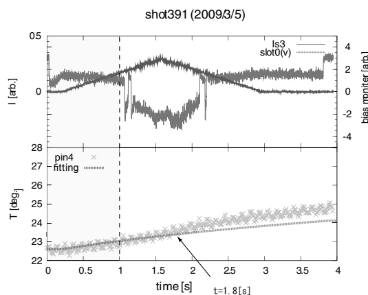
Fig. 2: Fitting results of a long discharge.
