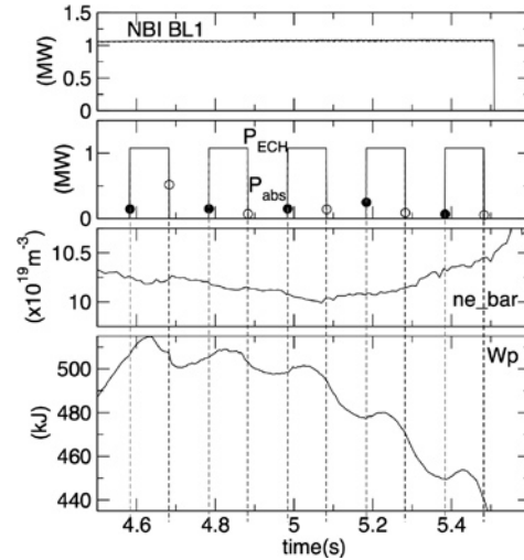
Figure 1 : (From the top) NBI #1 pulse, ECH pulses and absorbed power estimated from the change of the gradient of the stored energy, line integrated electron density, stored energy ( W_p ).
