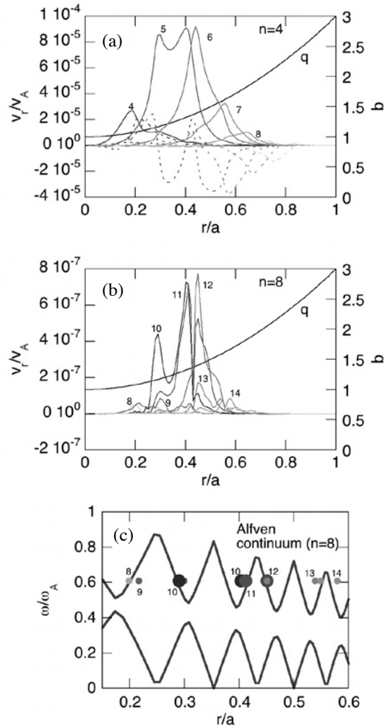
Fig. 1. Radial velocity profiles of the (a) n=4 and (b) n=8 modes, and (c) comparison of the peak location of each poloidal harmonic of the n=8 mode and n=8 shear Alfvén continuum.
