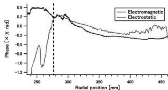
Fig. 2 Phase profiles of electromagnetic and electrostatic components.
