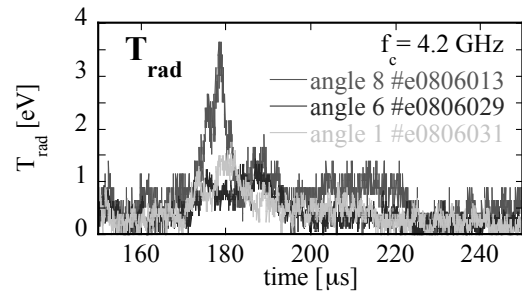
Fig. 2. Time evolution of radiation signal measured by the EBE system. Each curve with a different color shows T_{\text{rad}} for a different receiver angle \theta .
