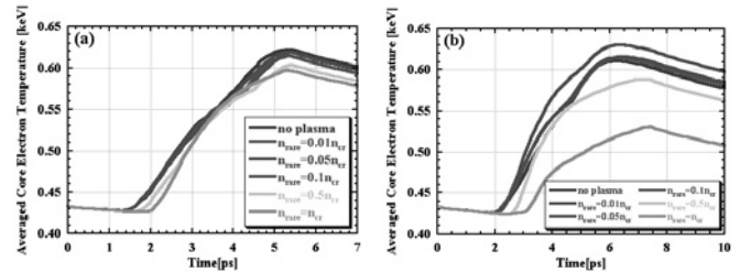
Fig.1. Time evolutions of averaged core electron temperature for (a) L_{\text{rare}}=150 and (b) 300\mu\text{m} .
