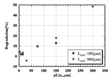
Fig.2. Degradations of electron temperature increment against the case without rarefied plasmas as a function of \rho L_{\text{rare}} \cdot \mu\text{m} for both L_{\text{rare}}=150 and 300\mu\text{m} .
