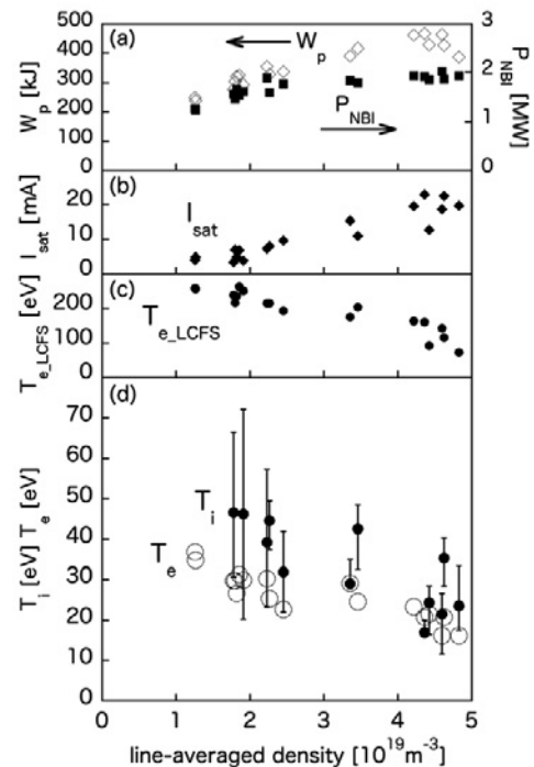
Fig. 2. Dependences of T_i and T_e in the LHD divertor legs on line-averaged density. (a) Plasma stored energy and NBI deposition power, (b) I_{sat} measured by the ISP, (c) T_e at LCFS measured by a YAG Thomson scattering system and (d) T_i and T_e measured by the ISP.
