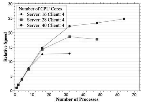
Fig. 3. Relative calculation speed vs. number of processes.
